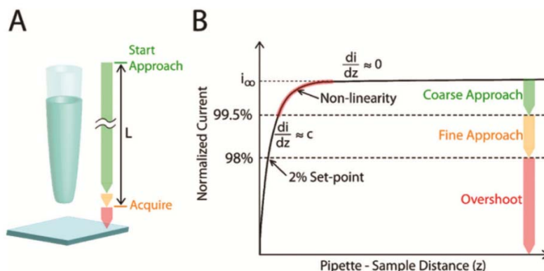
Figure 1: Measurement strategy for the Closed Loop-ARS mode. (A) Schematic of the proposed CL-ARS algorithm. (B) Normalized ion current through pipette, i/i_{\infty} , as a function of pipette-surface distance, z .
