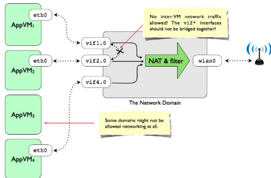
Figure 2. Networking overview.
